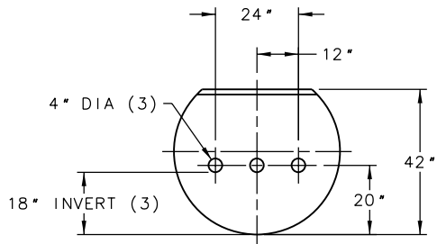
BAFFLE DETAIL
